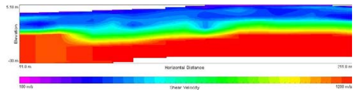
Example of a 2-dimensional ReMi Profile (with topography) Displaying Modeled Shear Wave Velocities
